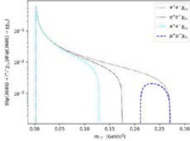
Fig. 4: The expected branching fractions for \psi(3686) \rightarrow \ell^+\ell^-\chi_{c0,1,2} as a function of di-lepton invariant mass spectrum for both electron-pair and muon-pair decay channels.
