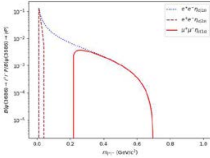
Fig. 2: The branching fraction ratio \frac{B(\psi(3686) \rightarrow \ell^+ \ell^- \eta_c(1S,2S))}{B(\psi(3686) \rightarrow \gamma \eta_c(1S,2S))} versus m_{\ell^+ \ell^-} for e^+ e^- (blue) and \mu^+ \mu^- (red) channels.
