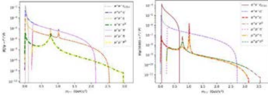
Fig. 1: The expected branching fractions of J/\psi \rightarrow \ell^+\ell^-P (left) and \psi(3686) \rightarrow \ell^+\ell^-P (right) as a function of m_{\ell^+\ell^-} including the intermediate resonances of \rho , \omega , and \phi .
